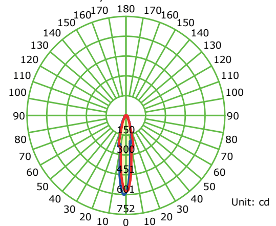
Luminous Intensity Distribution Curve - Green
